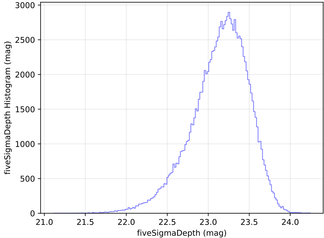
internal_u_expt30_nscale1.0v3.4_10yrs WFD u band: fiveSigmaDepth Histogram
