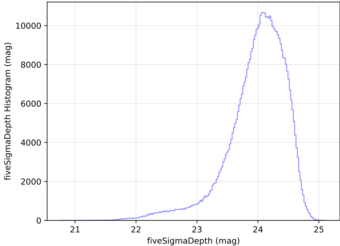
internal_u_expt30_nscale1.0v3.4_10yrs WFD r band: fiveSigmaDepth Histogram
