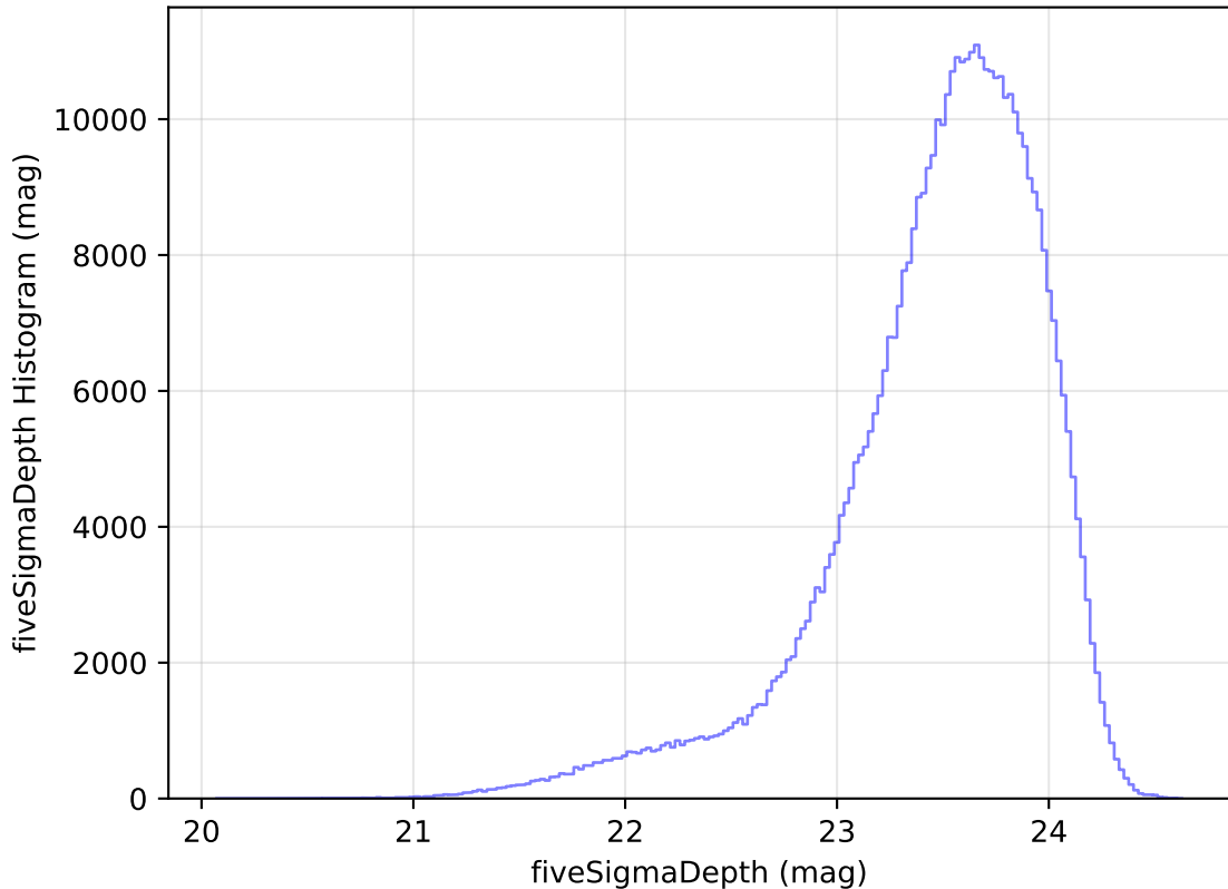
internal_u_expt30_nscale1.0v3.4_10yrs WFD i band: fiveSigmaDepth Histogram
