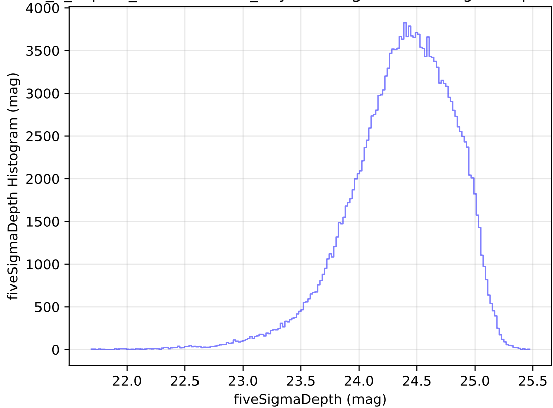
internal_u_expt30_nscale1.0v3.4_10yrs WFD g band: fiveSigmaDepth Histogram
