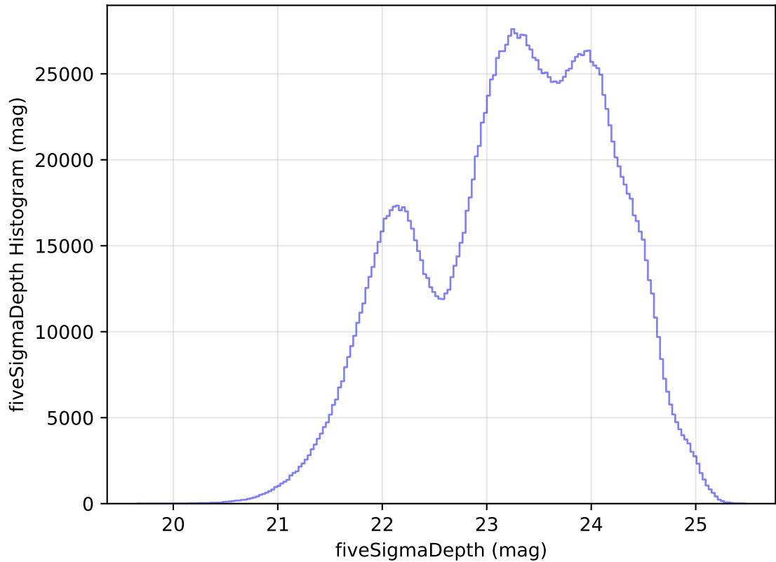
internal_u_expt30_nscale1.0v3.4_10yrs WFD all bands: fiveSigmaDepth Histogram
