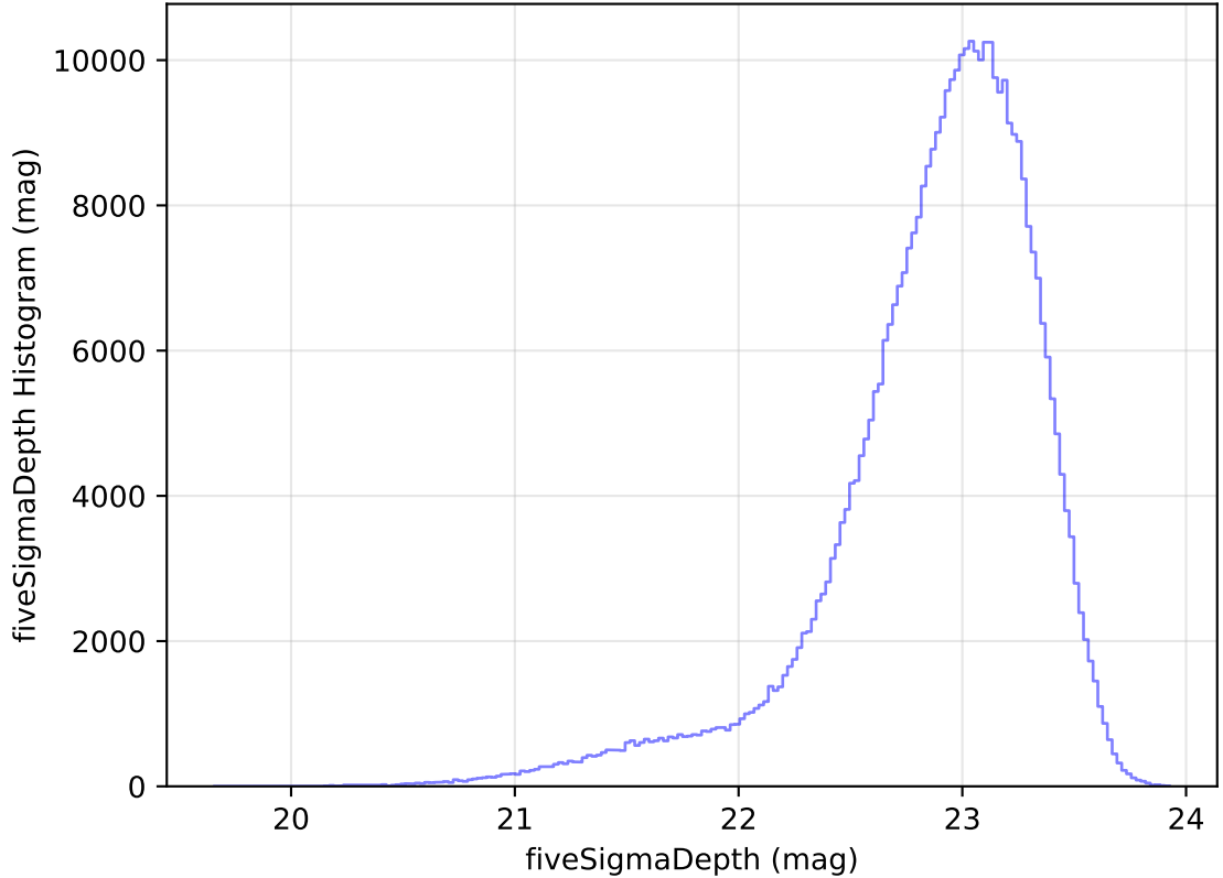
internal_u_expt30_nscale1.0v3.4_10yrs All sky z band: fiveSigmaDepth Histogram
