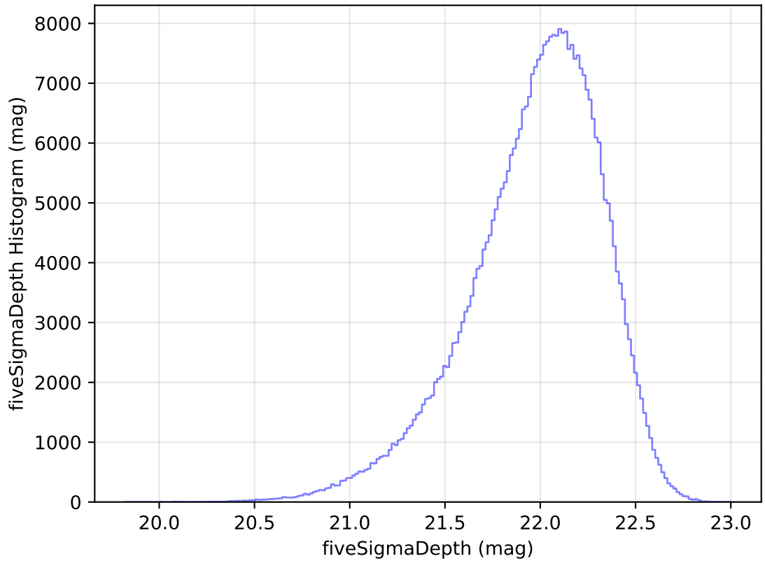
internal_u_expt30_nscale1.0v3.4_10yrs All sky y band: fiveSigmaDepth Histogram
