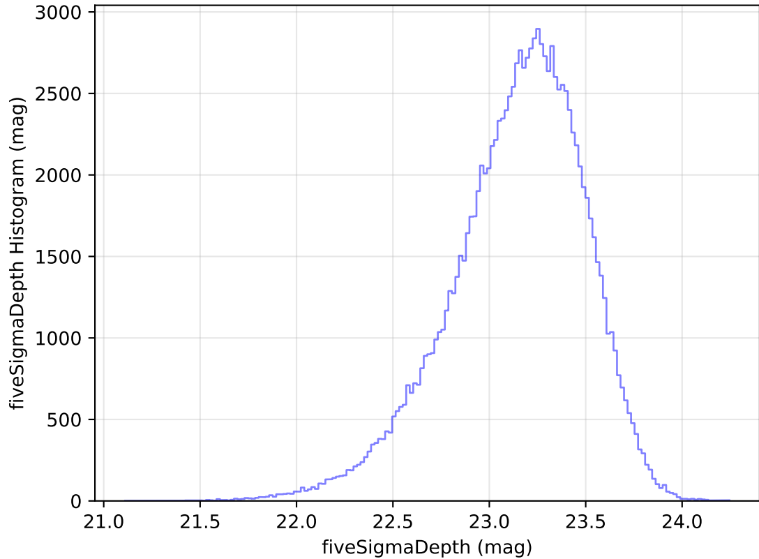
internal_u_expt30_nscale1.0v3.4_10yrs All sky u band: fiveSigmaDepth Histogram
