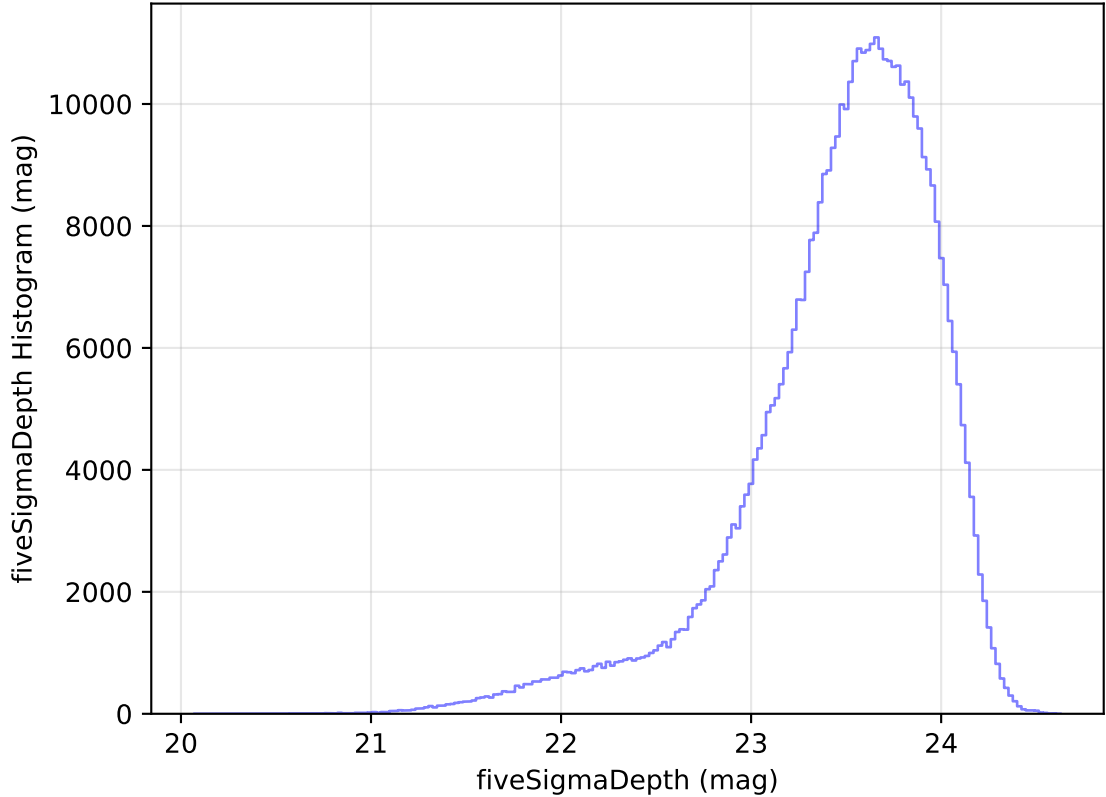
internal_u_expt30_nscale1.0v3.4_10yrs All sky i band: fiveSigmaDepth Histogram
