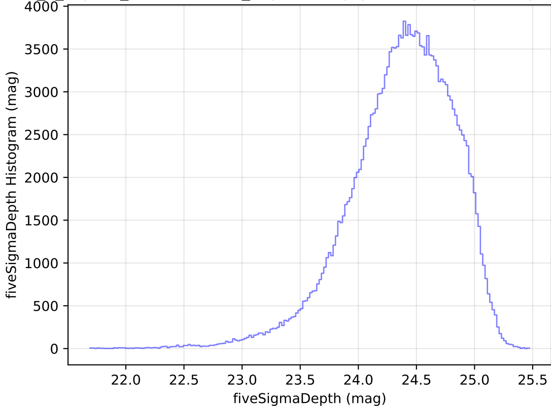
internal_u_expt30_nscale1.0v3.4_10yrs All sky g band: fiveSigmaDepth Histogram
