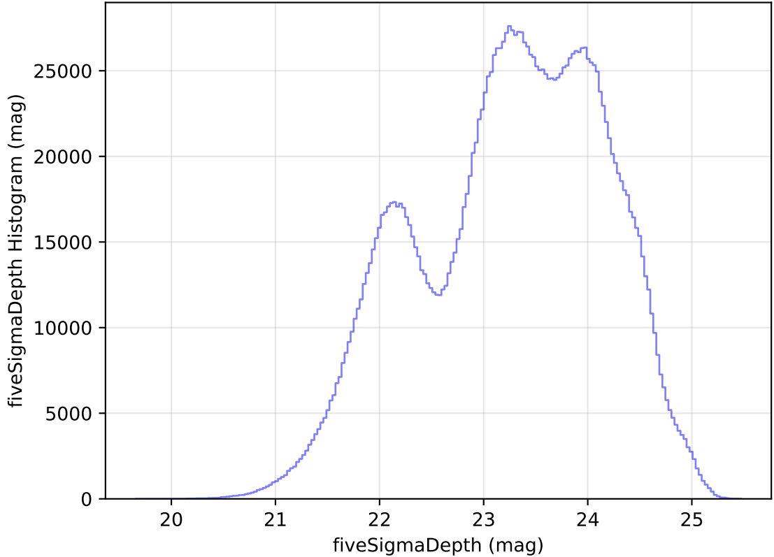
internal_u_expt30_nscale1.0v3.4_10yrs All sky all bands: fiveSigmaDepth Histogram
