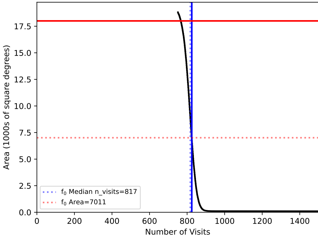
internal_u_expt30_nscale1.0v3.4_10yrs WFD: fO
