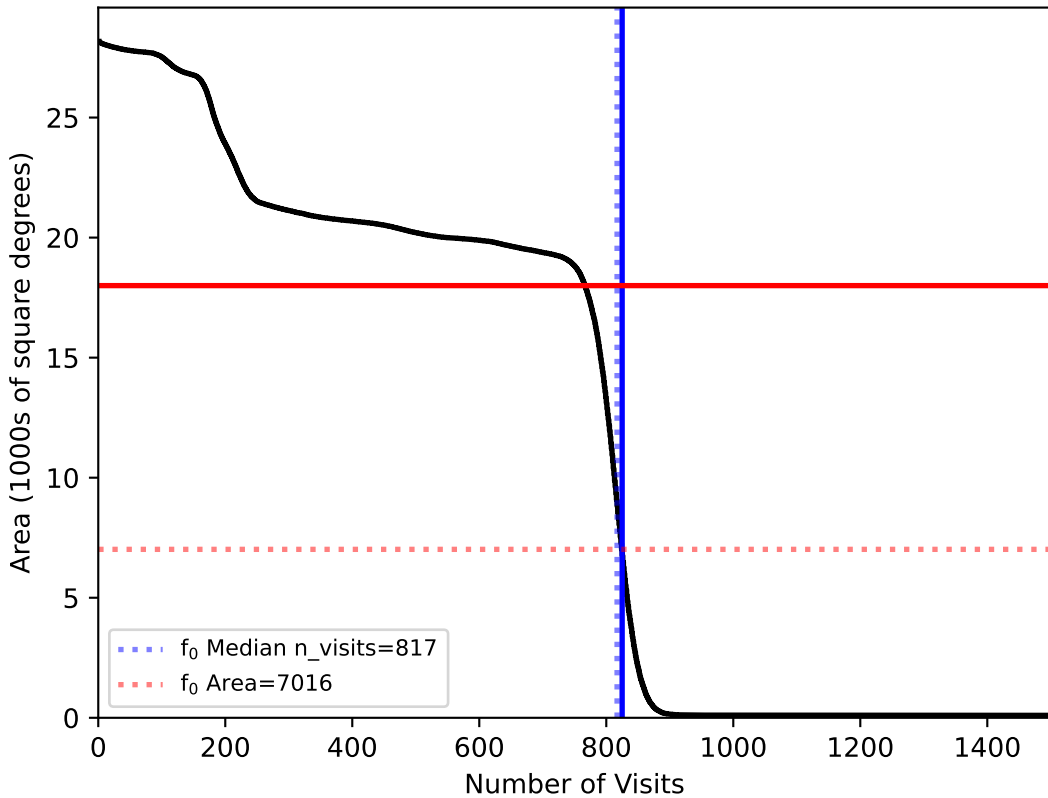
internal_u_expt30_nscale1.0v3.4_10yrs All sky: f0
