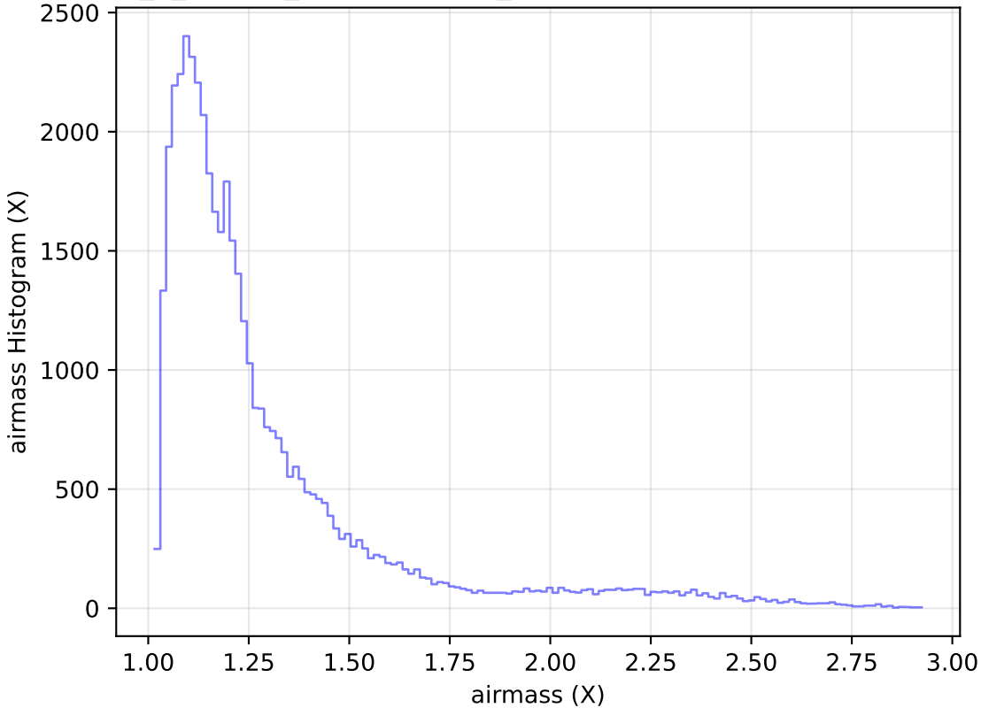
internal_u_expt30_nscale1.0v3.4_10yrs Yr 1 z band: airmass Histogram
