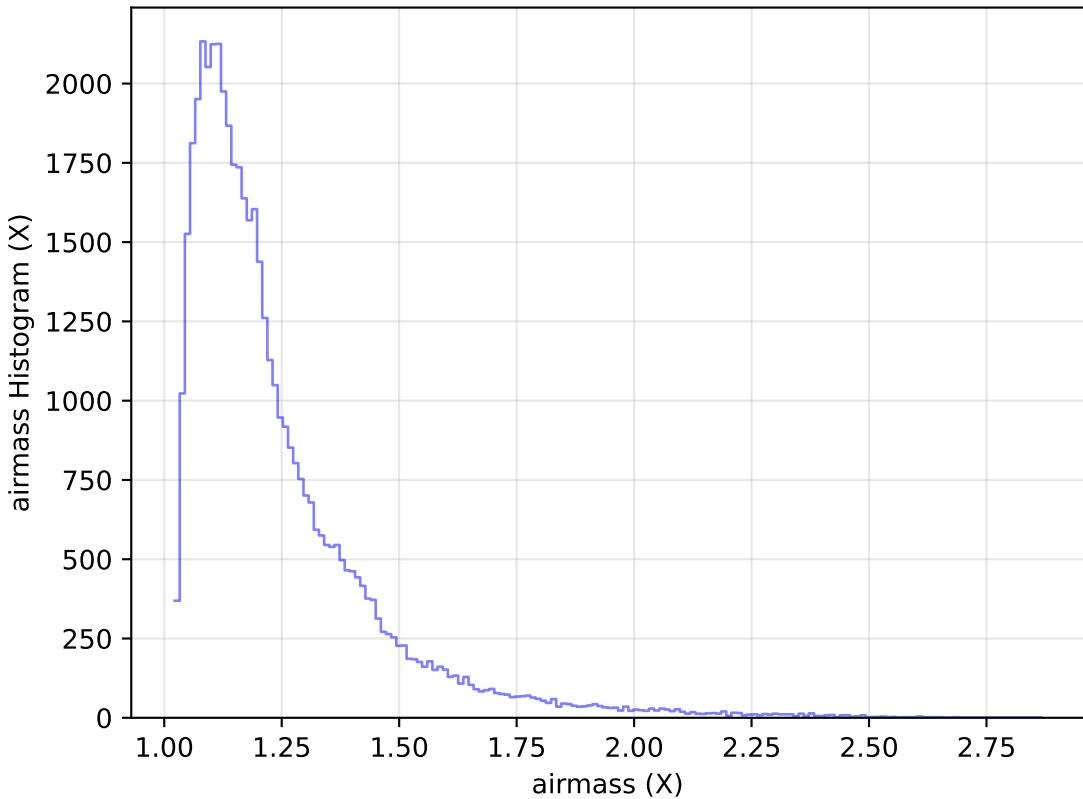
internal_u_expt30_nscale1.0v3.4_10yrs Yr 1 y band: airmass Histogram
