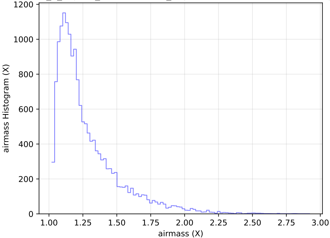
internal_u_expt30_nscale1.0v3.4_10yrs Yr 1 u band: airmass Histogram
