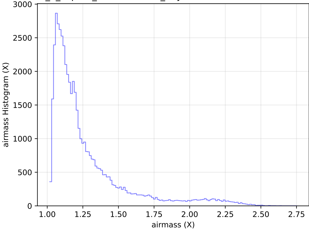
internal_u_expt30_nscale1.0v3.4_10yrs Yr 1 r band: airmass Histogram
