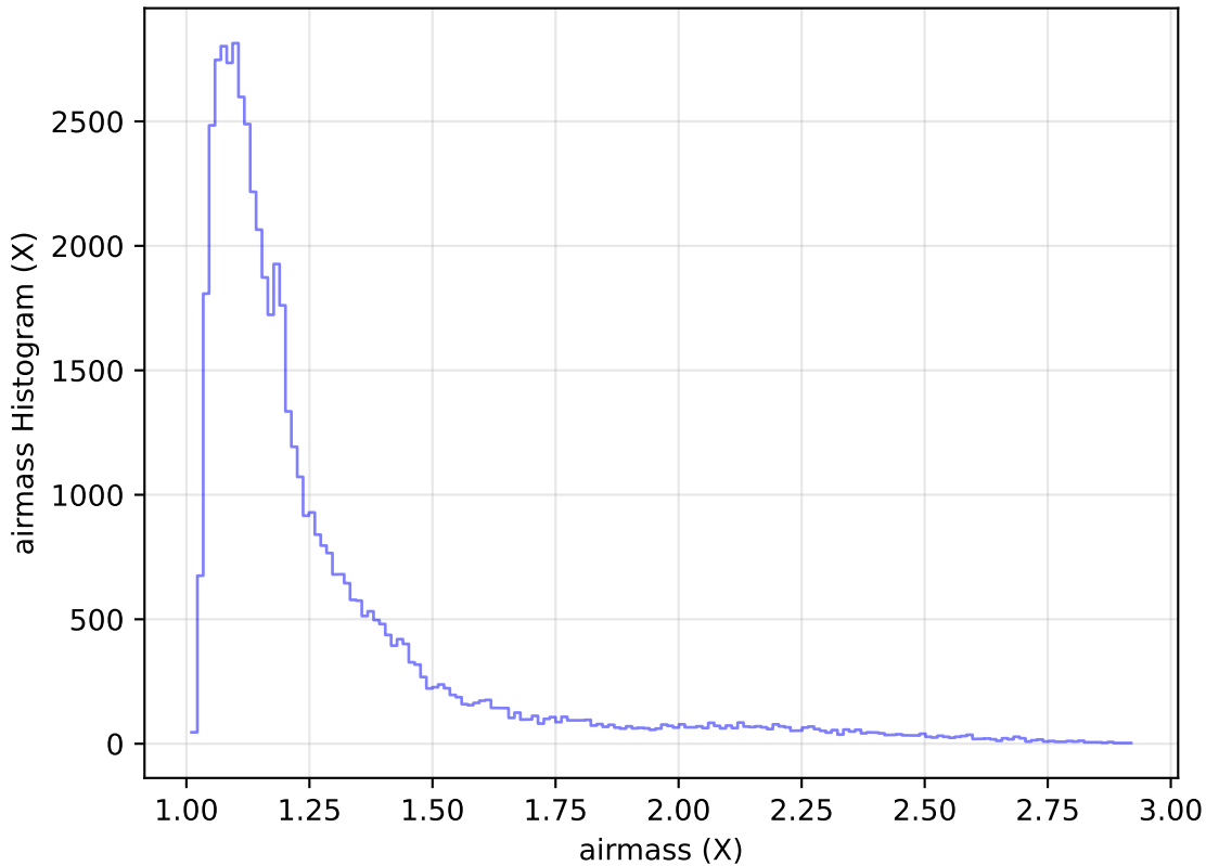
internal_u_expt30_nscale1.0v3.4_10yrs Yr 1 i band: airmass Histogram
