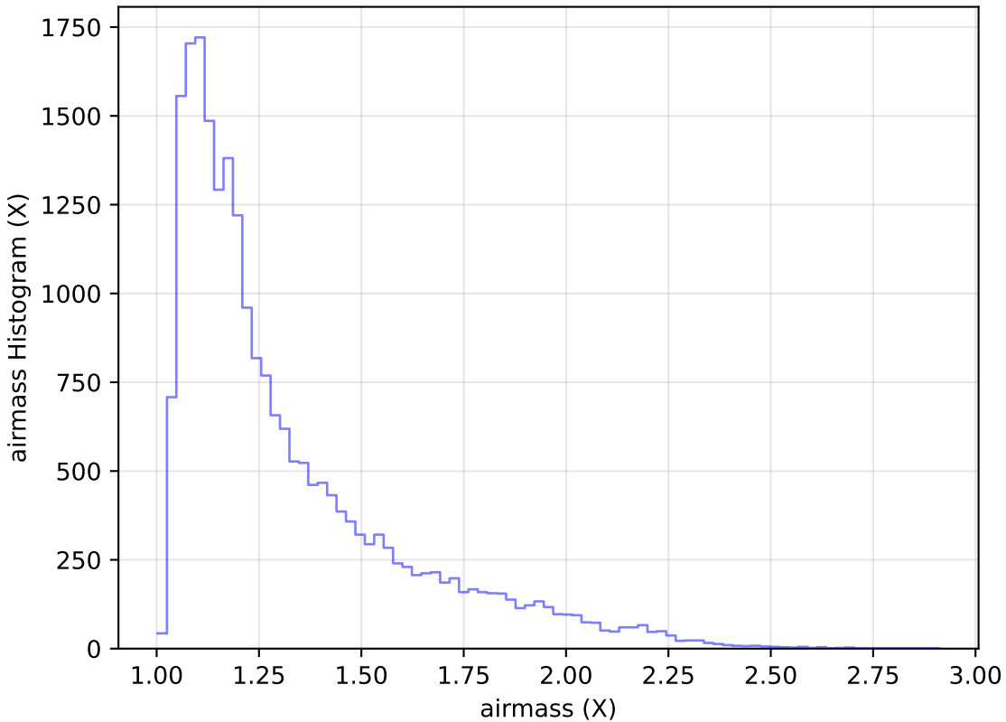
internal_u_expt30_nscale1.0v3.4_10yrs Yr 1 g band: airmass Histogram
