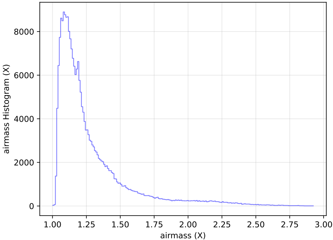
internal_u_expt30_nscale1.0v3.4_10yrs Yr 1 all bands: airmass Histogram
