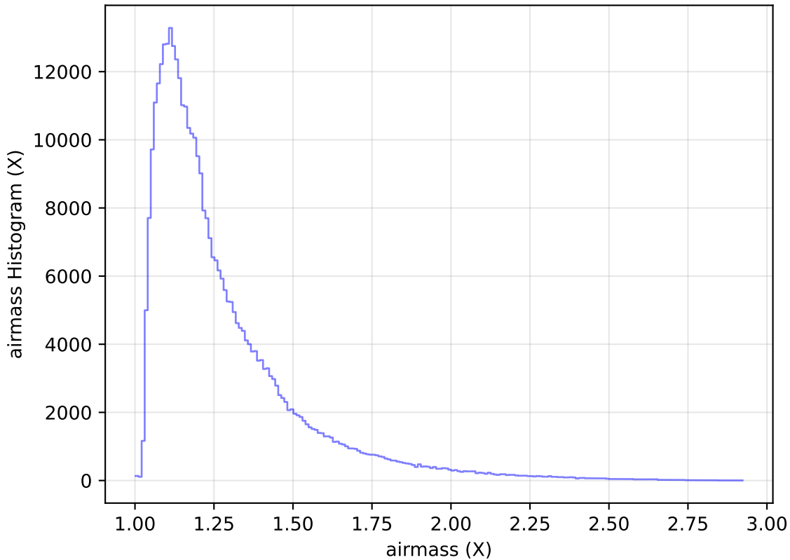
internal_u_expt30_nscale1.0v3.4_10yrs WFD y band: airmass Histogram
