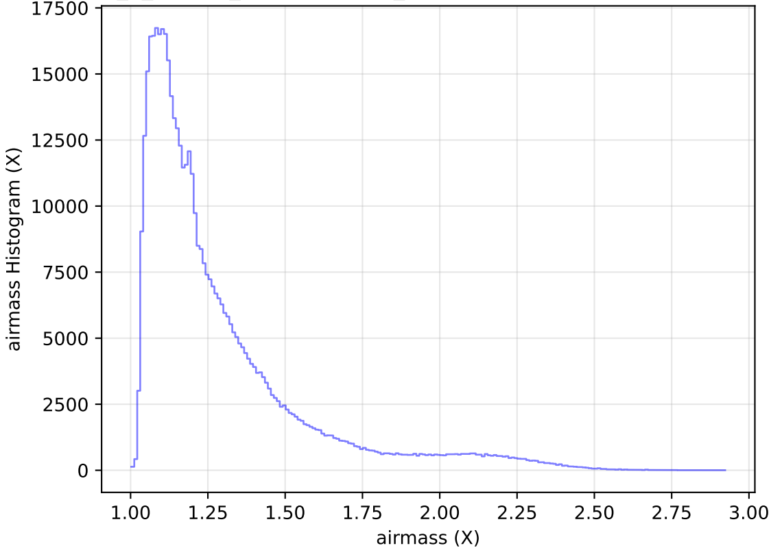
internal_u_expt30_nscale1.0v3.4_10yrs WFD r band: airmass Histogram
