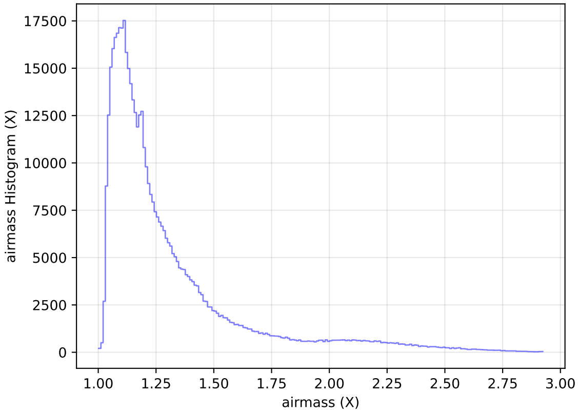
internal_u_expt30_nscale1.0v3.4_10yrs WFD i band: airmass Histogram
