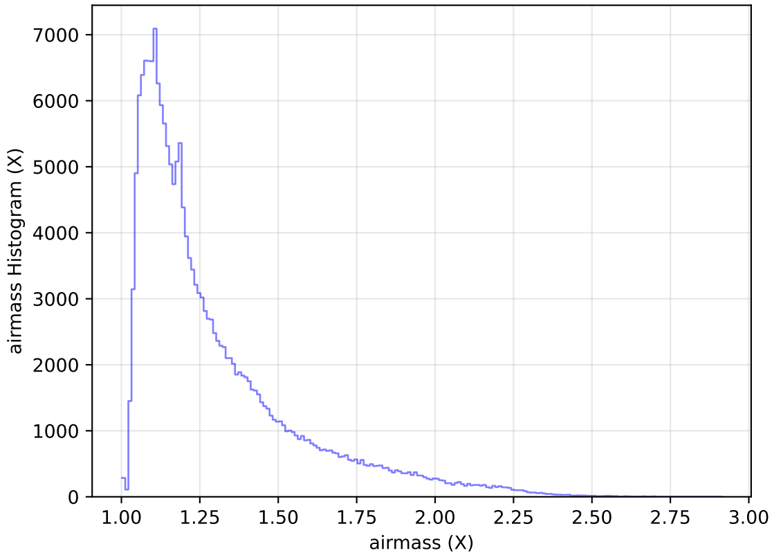
internal_u_expt30_nscale1.0v3.4_10yrs WFD g band: airmass Histogram
