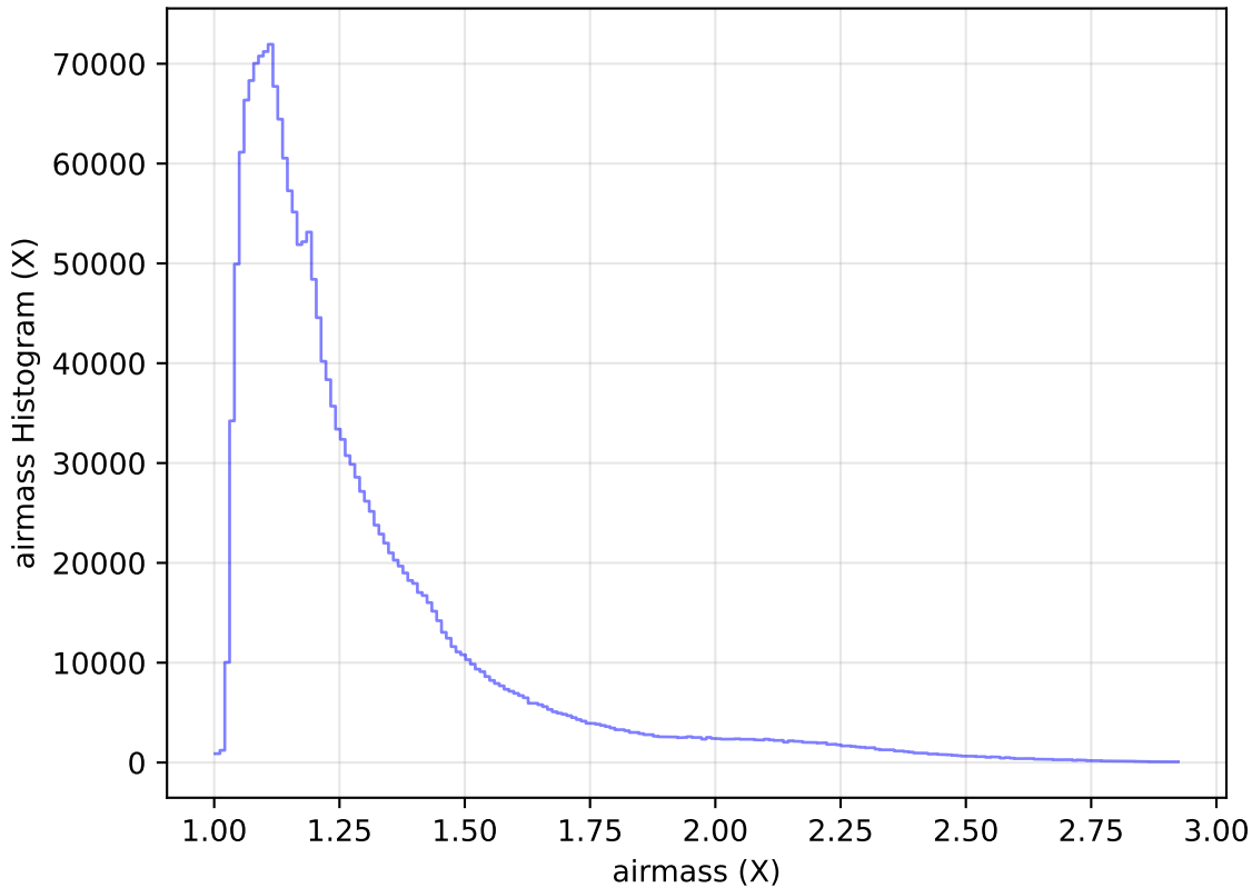
internal_u_expt30_nscale1.0v3.4_10yrs WFD all bands: airmass Histogram
