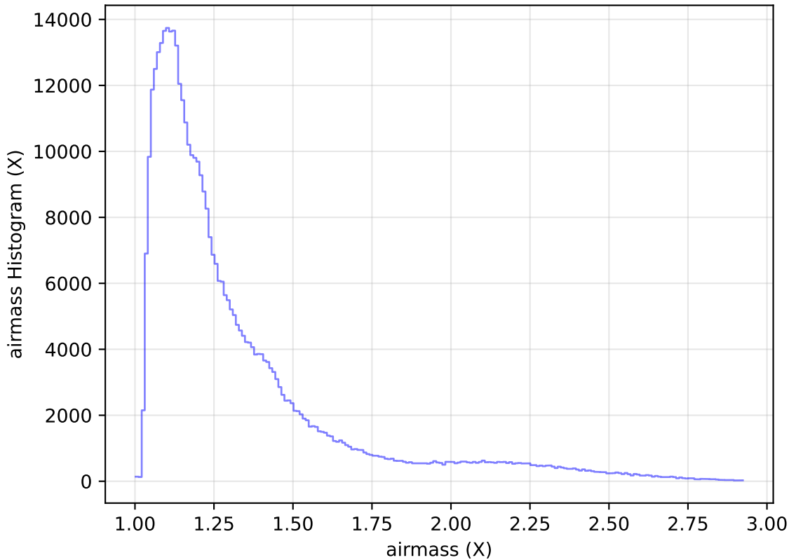
internal_u_expt30_nscale1.0v3.4_10yrs All sky z band: airmass Histogram
