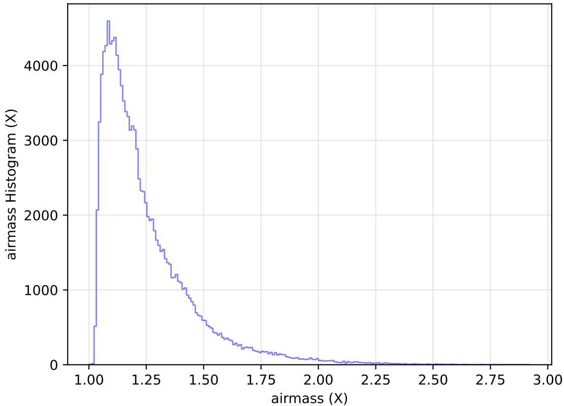
internal_u_expt30_nscale1.0v3.4_10yrs All sky u band: airmass Histogram
