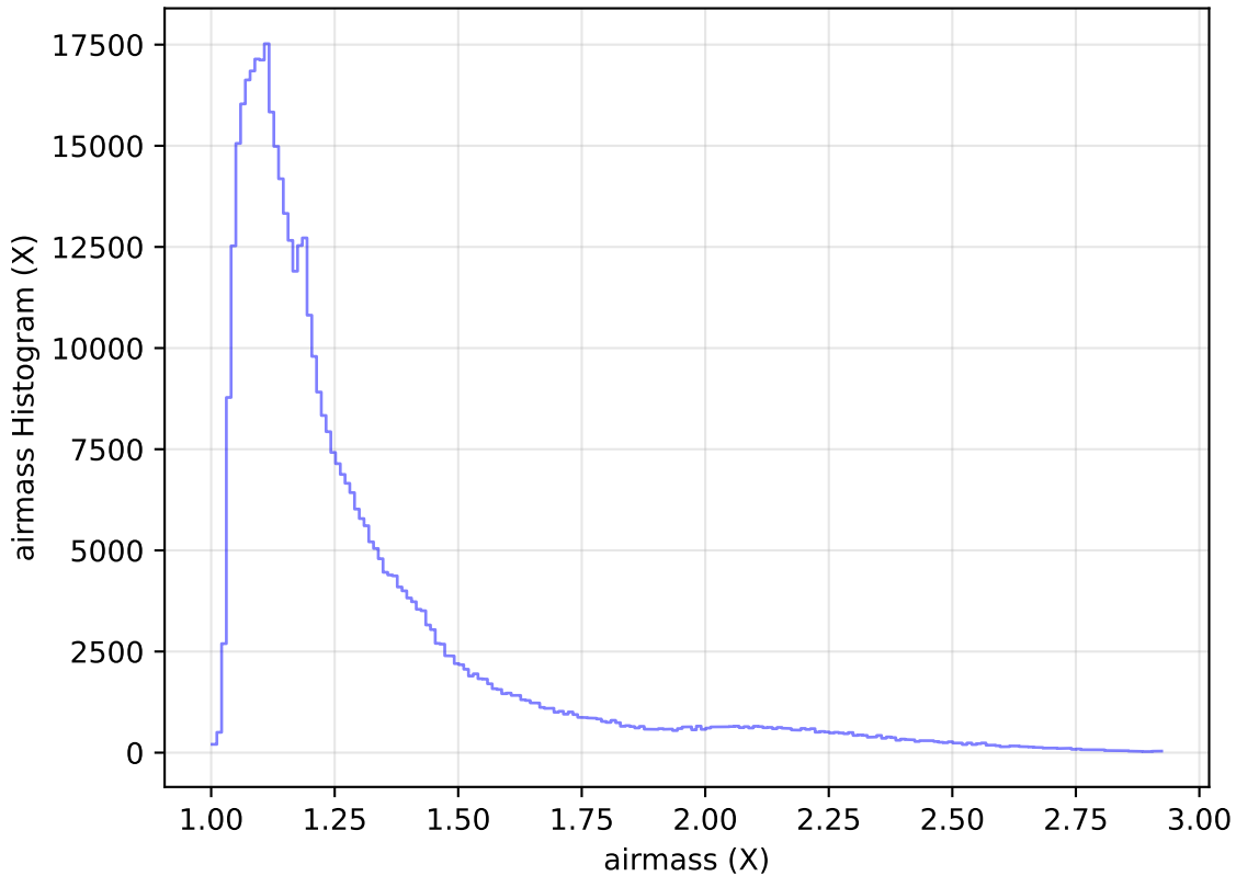
internal_u_expt30_nscale1.0v3.4_10yrs All sky i band: airmass Histogram
