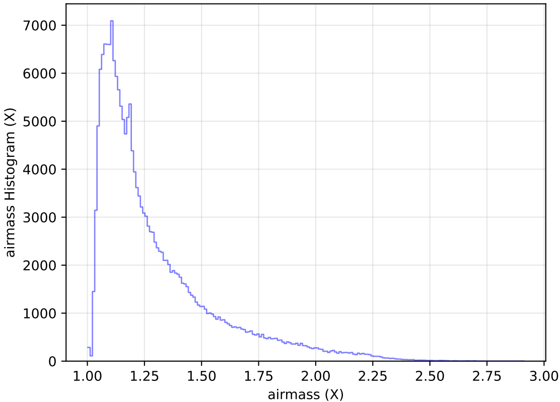
internal_u_expt30_nscale1.0v3.4_10yrs All sky g band: airmass Histogram
