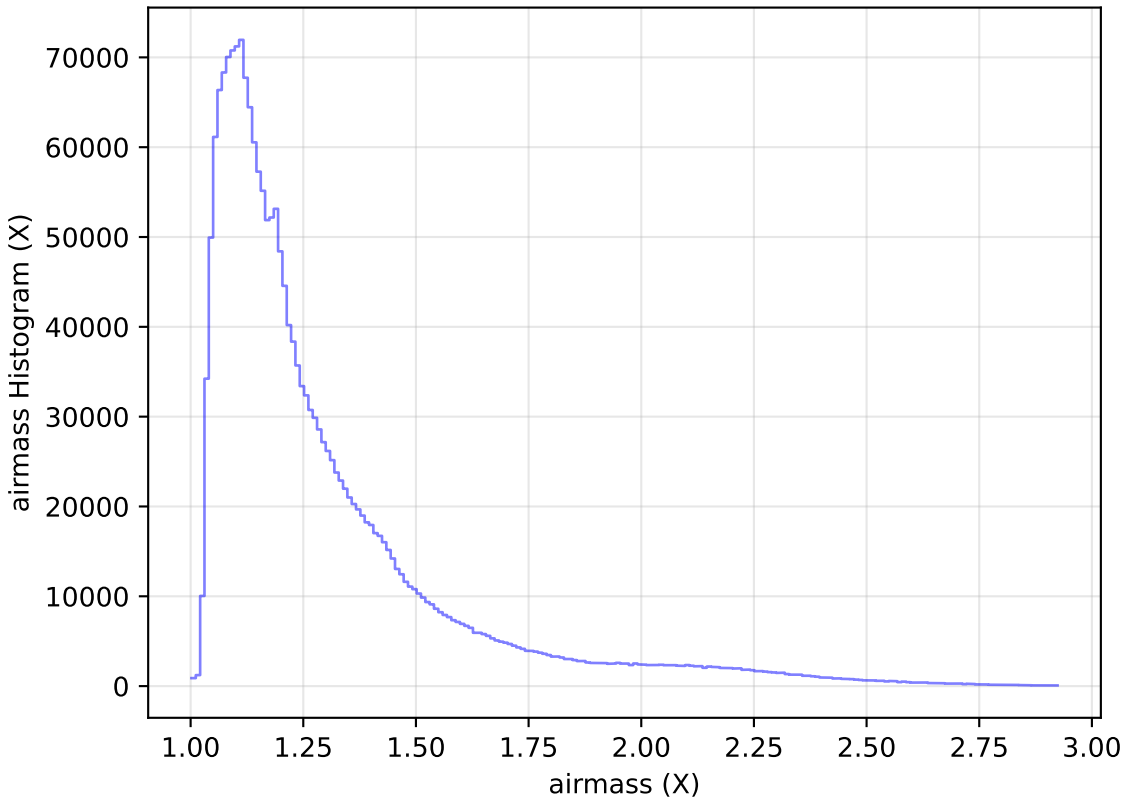
internal_u_expt30_nscale1.0v3.4_10yrs All sky all bands: airmass Histogram
