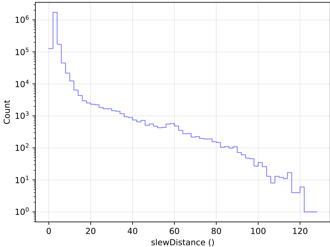
internal_u_expt30_nscale1.0v3.4_10yrs All visits: Slew Distance Histogram
