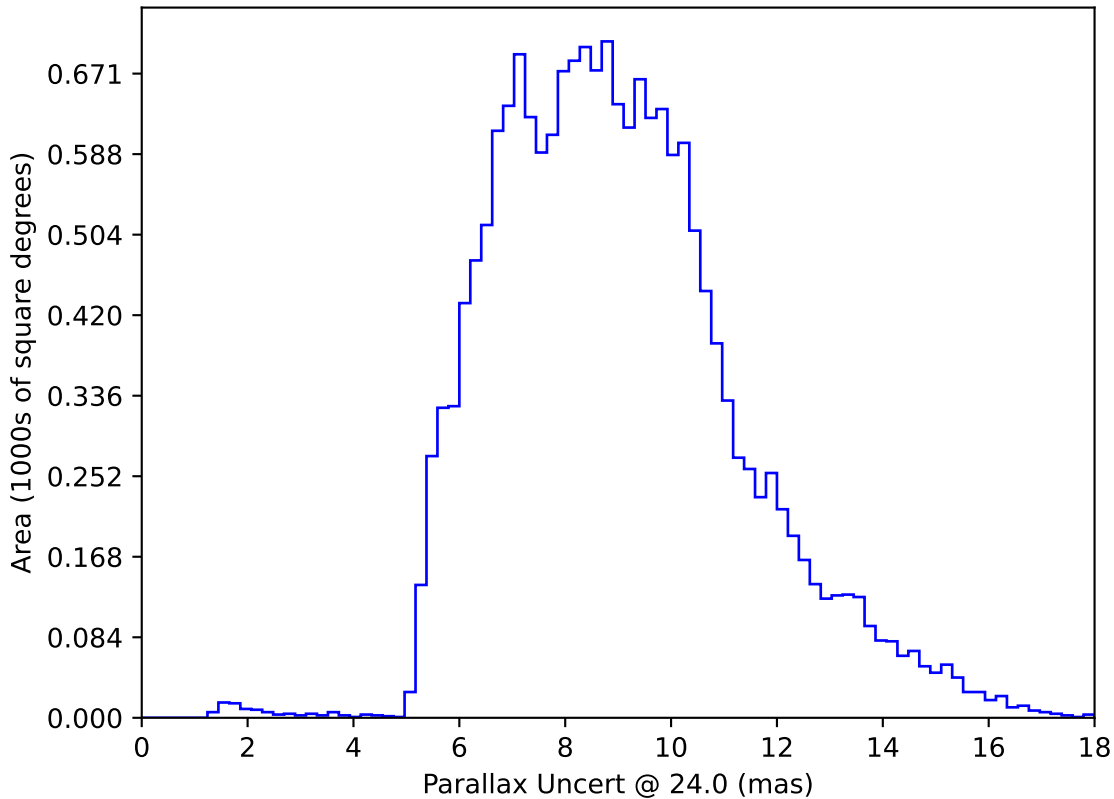
internal_u_expt30_nscale1.0v3.4_10yrs WFD: Parallax Uncert @ 24.0
