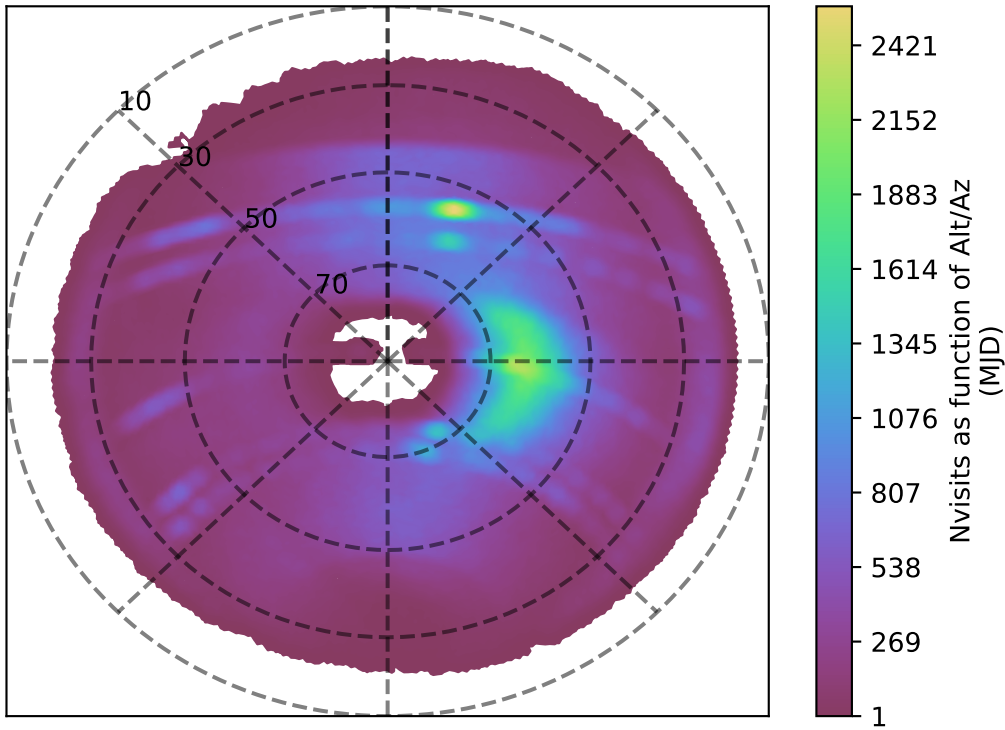
internal_u_expt30_nscale1.0v3.4_10yrs z band: Nvisits as function of Alt/Az
