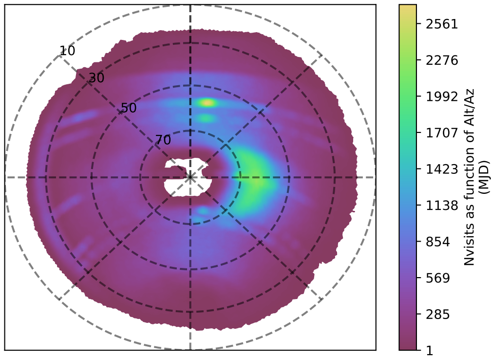
internal_u_expt30_nscale1.0v3.4_10yrs r band: Nvisits as function of Alt/Az
