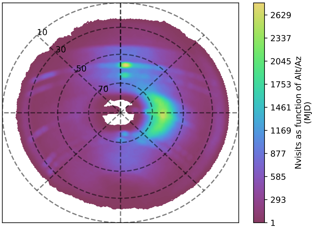
internal_u_expt30_nscale1.0v3.4_10yrs i band: Nvisits as function of Alt/Az
