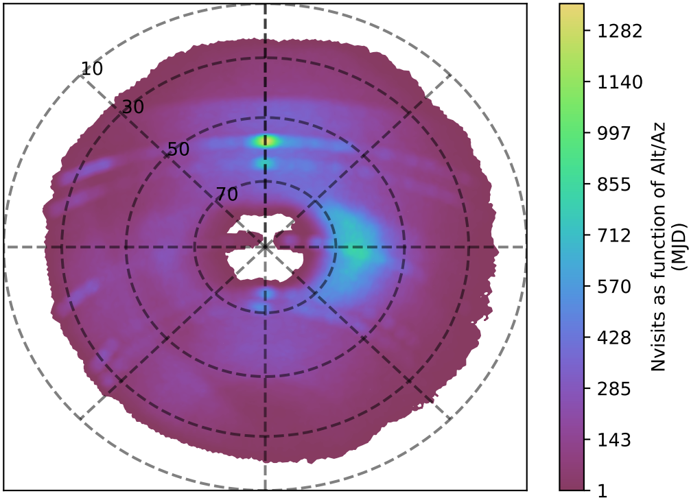
internal_u_expt30_nscale1.0v3.4_10yrs g band: Nvisits as function of Alt/Az
