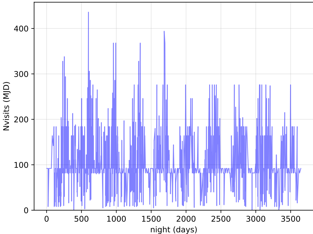
internal_u_expt30_nscale1.0v3.4_10yrs DDF: Nvisits
