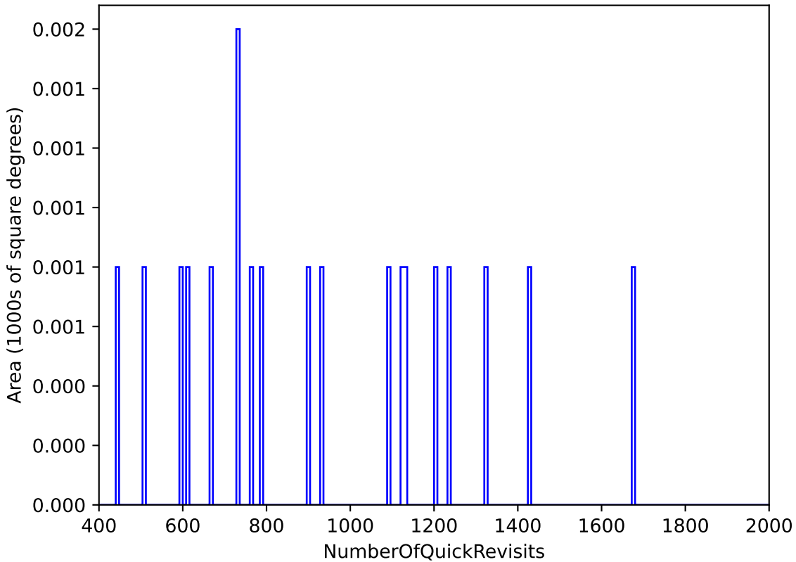
internal_u_expt30_nscale1.0v3.4_10yrs All sky: NumberOfQuickRevisits
