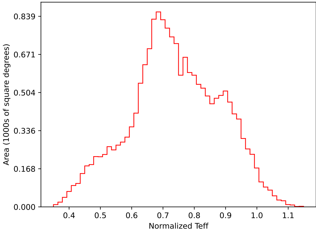
internal_u_expt30_nscale1.0v3.4_10yrs WFD i band: Normalized Teff
