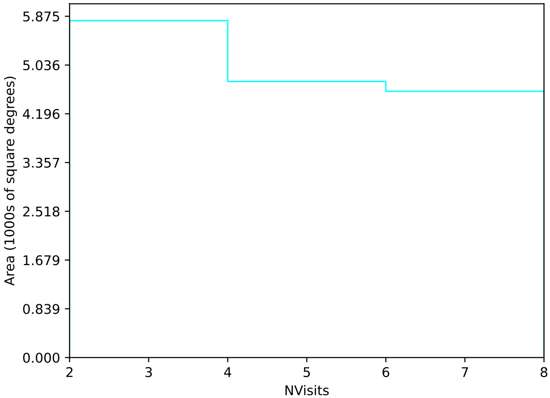
internal_u_expt30_nscale1.0v3.4_10yrs Yr 3-4 u band: NVisits
