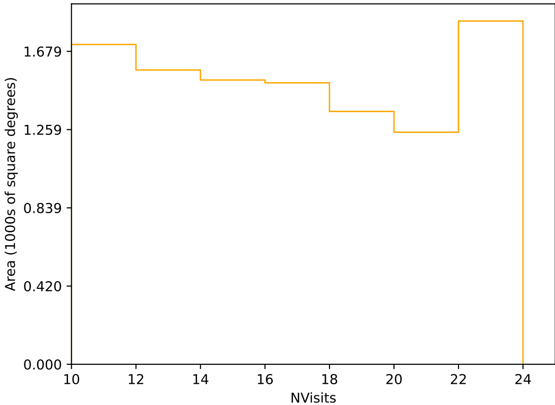
internal_u_expt30_nscale1.0v3.4_10yrs Yr 3-4 r band: NVisits
