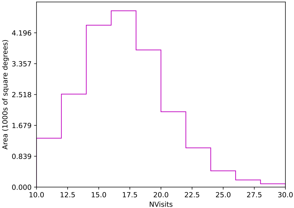
internal_u_expt30_nscale1.0v3.4_10yrs Yr 1 z band: NVisits
