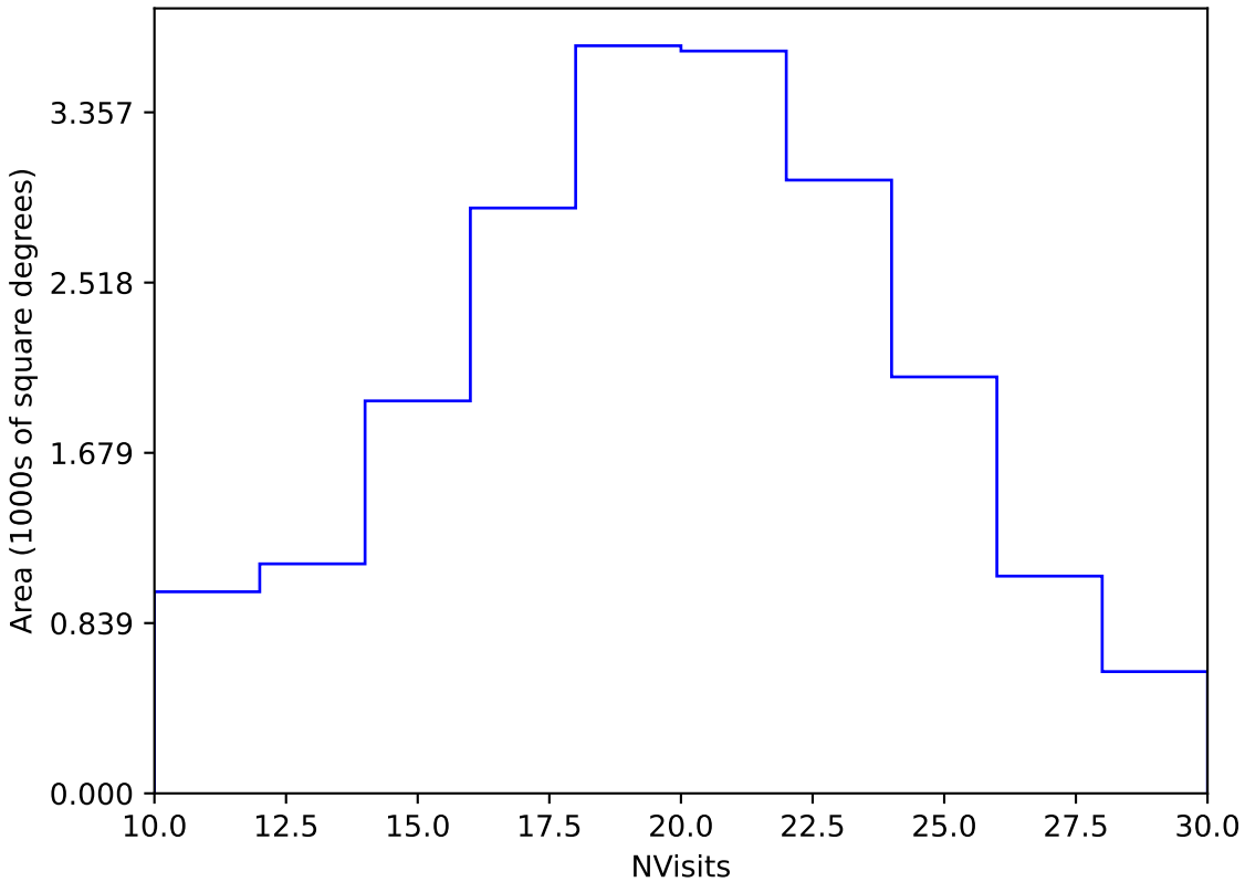
internal_u_expt30_nscale1.0v3.4_10yrs Yr 1 y band: NVisits
