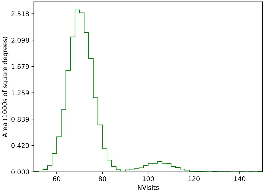
internal_u_expt30_nscale1.0v3.4_10yrs WFD g band: NVisits
