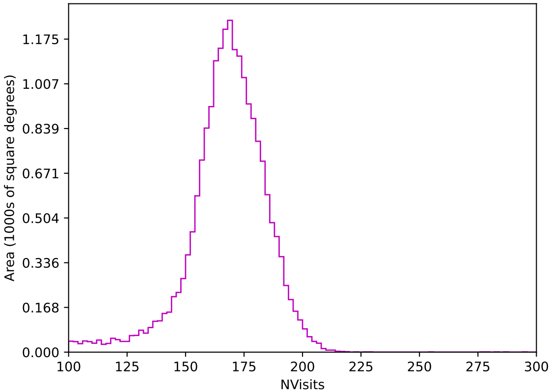
internal_u_expt30_nscale1.0v3.4_10yrs All sky z band: NVisits
