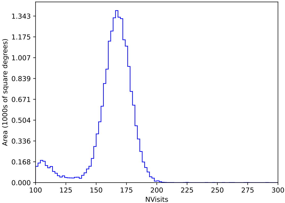
internal_u_expt30_nscale1.0v3.4_10yrs All sky y band: NVisits
