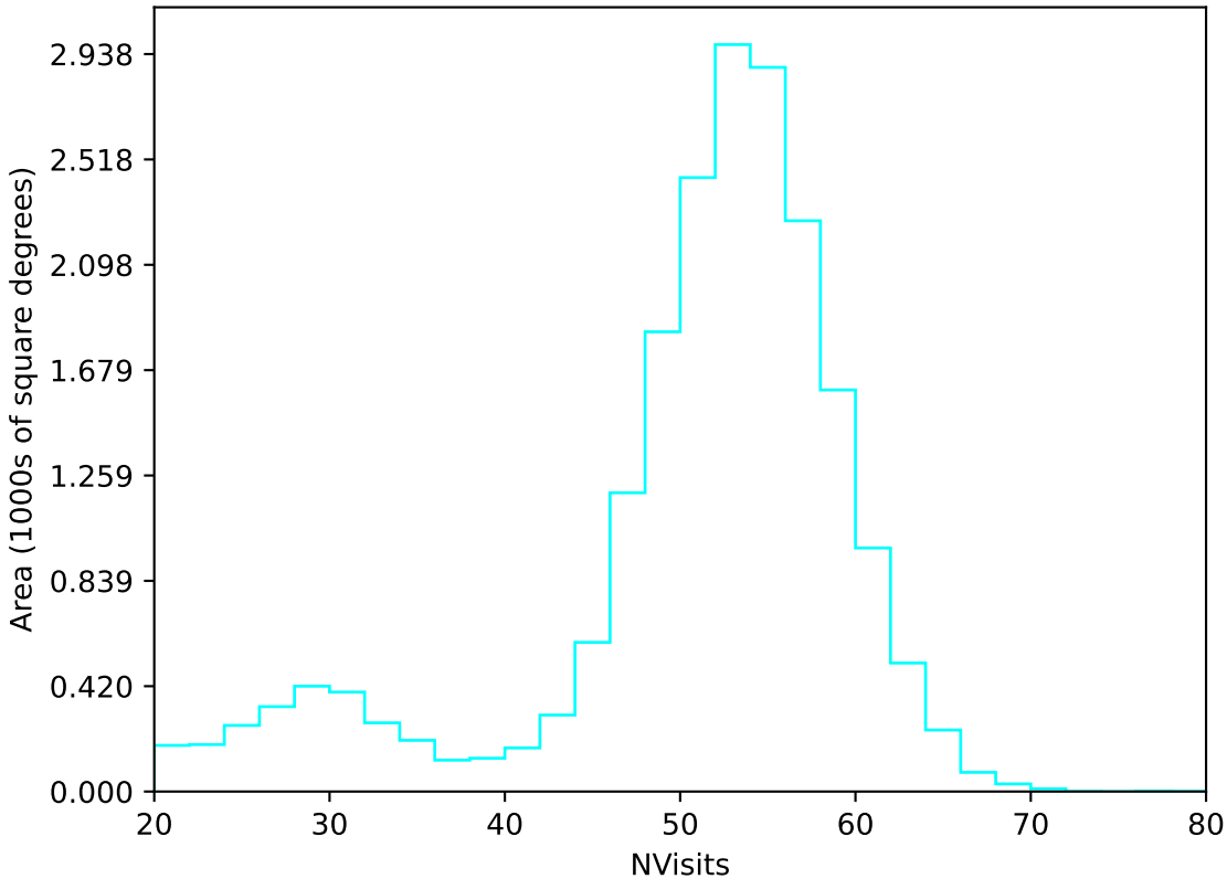
internal_u_expt30_nscale1.0v3.4_10yrs All sky u band: NVisits
