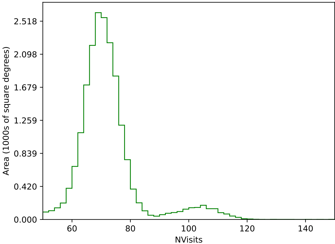
internal_u_expt30_nscale1.0v3.4_10yrs All sky g band: NVisits
