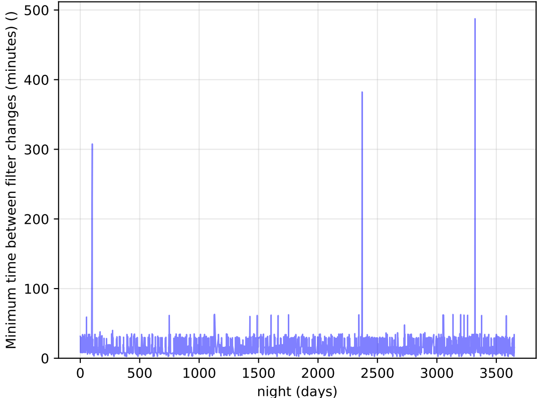
internal_u_expt30_nscale1.0v3.4_10yrs Per Night: Minimum time between filter changes (minutes)
