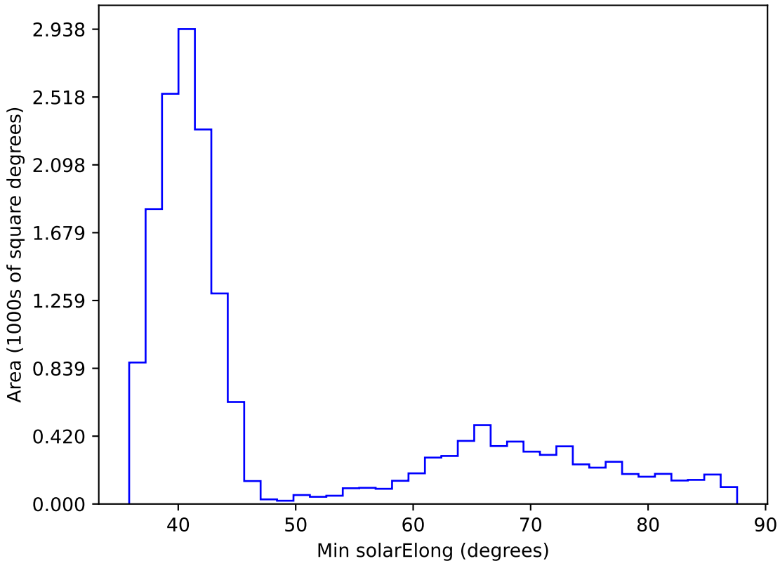
internal_u_expt30_nscale1.0v3.4_10yrs WFD i band: Min solarElong
